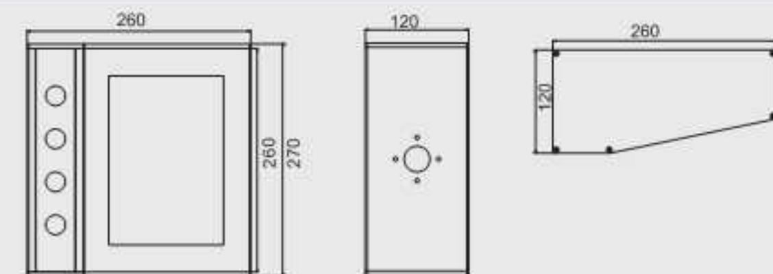
Model:LPN260 Size:120x260xL(mm) L size custom-made
