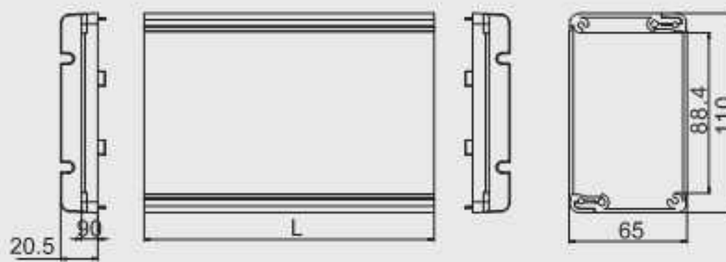
Model:LPV110 Size:65x110xL(mm) L size custom-made
