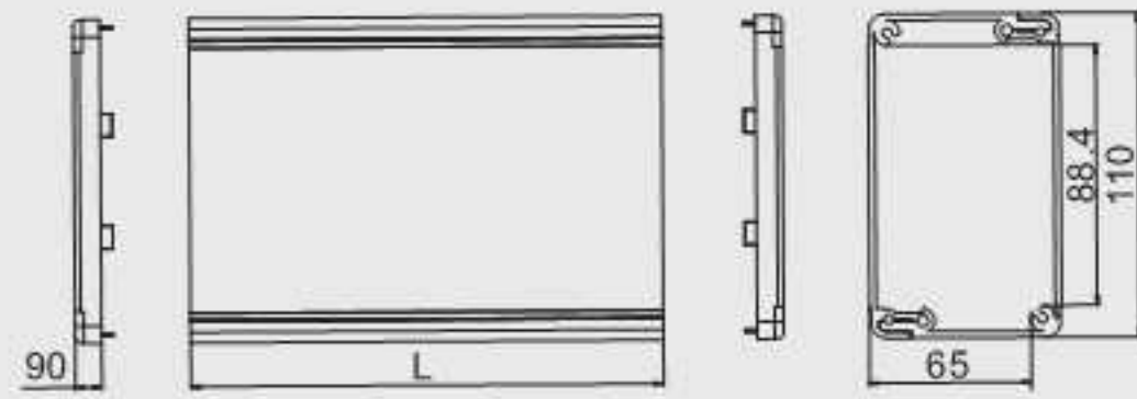
Model:LPN110 Size:65x110xL(mm) L size custom-made
