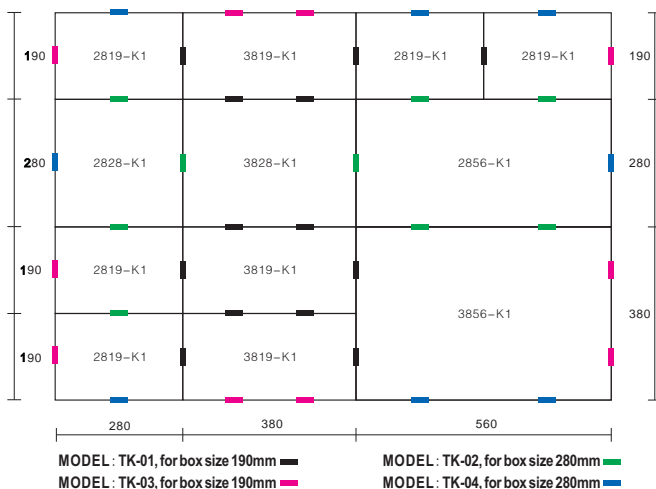
Joint plastic board MODEL: TK-01, for box size 190mm
