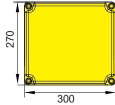
Model:TJ-AG-2730 Size:270x300x145mm
