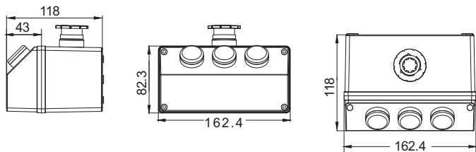
Model:TJ-T03 Size:160x82x118mm
